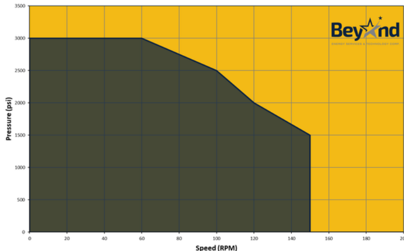
ARES 3078/POSEIDON 3078 Maximum Dynamic Operational Limits
