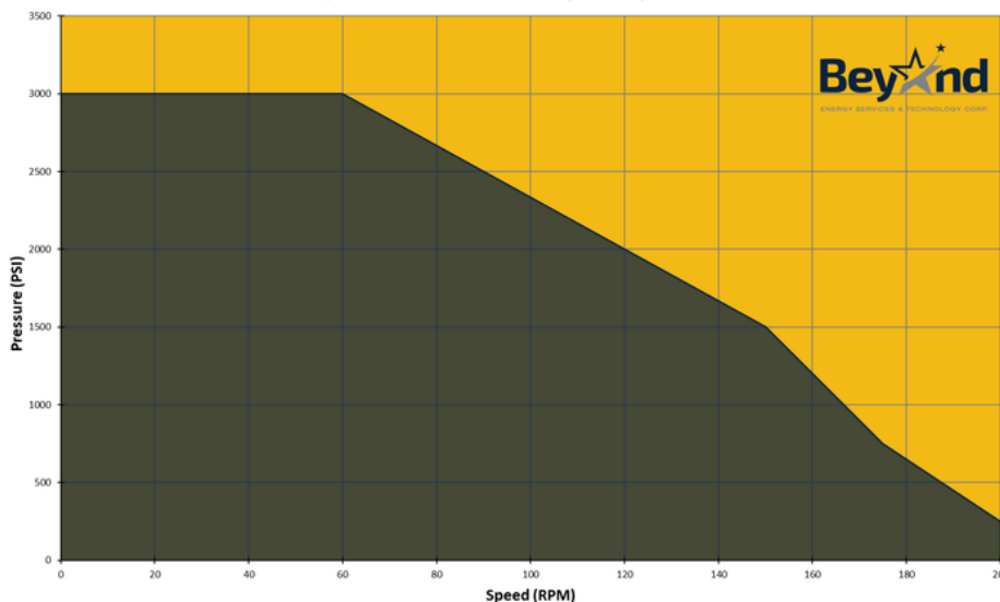
ARES 3090/POSEIDON 3090 Maximum Dynamic Operational Limits
