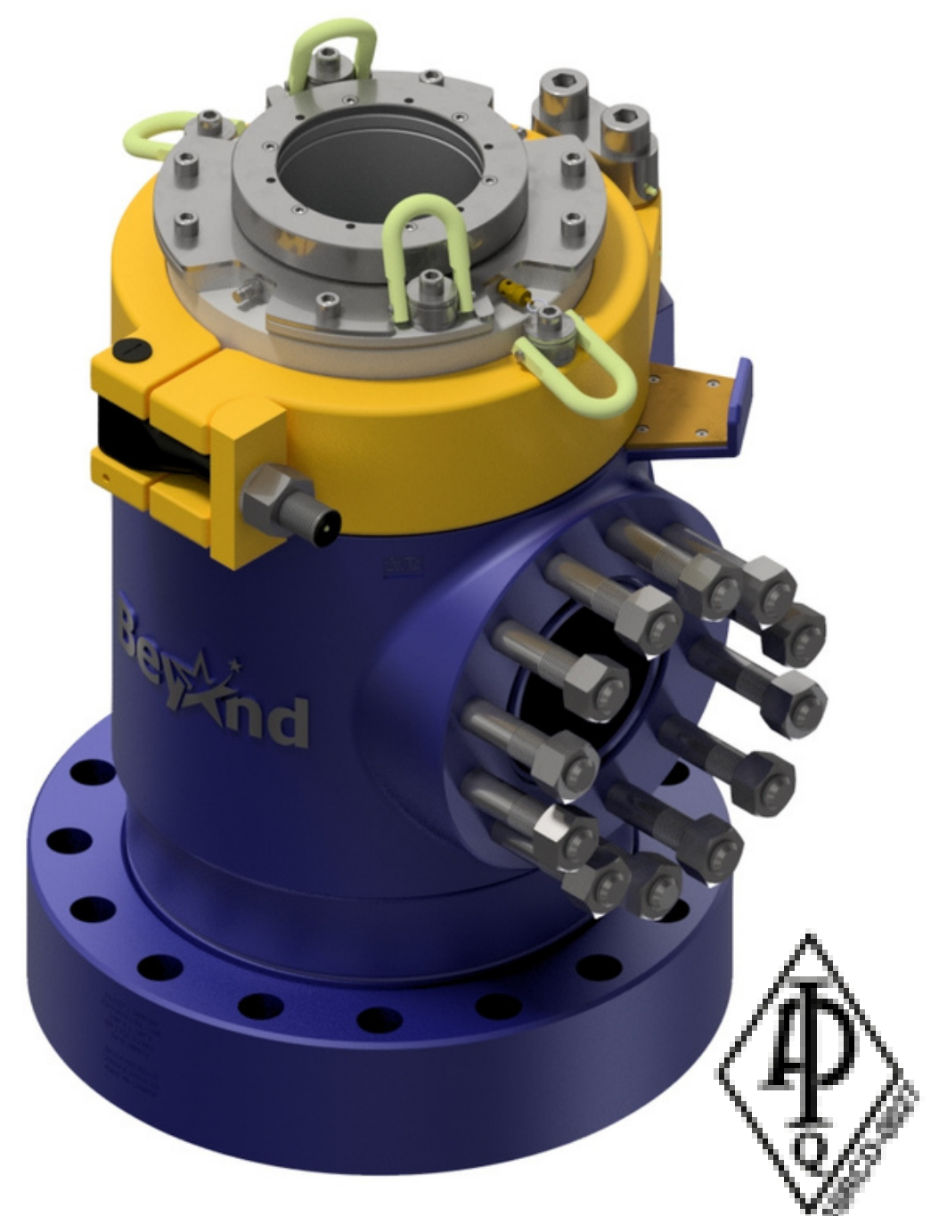
TITAN 3 RCD BODY
