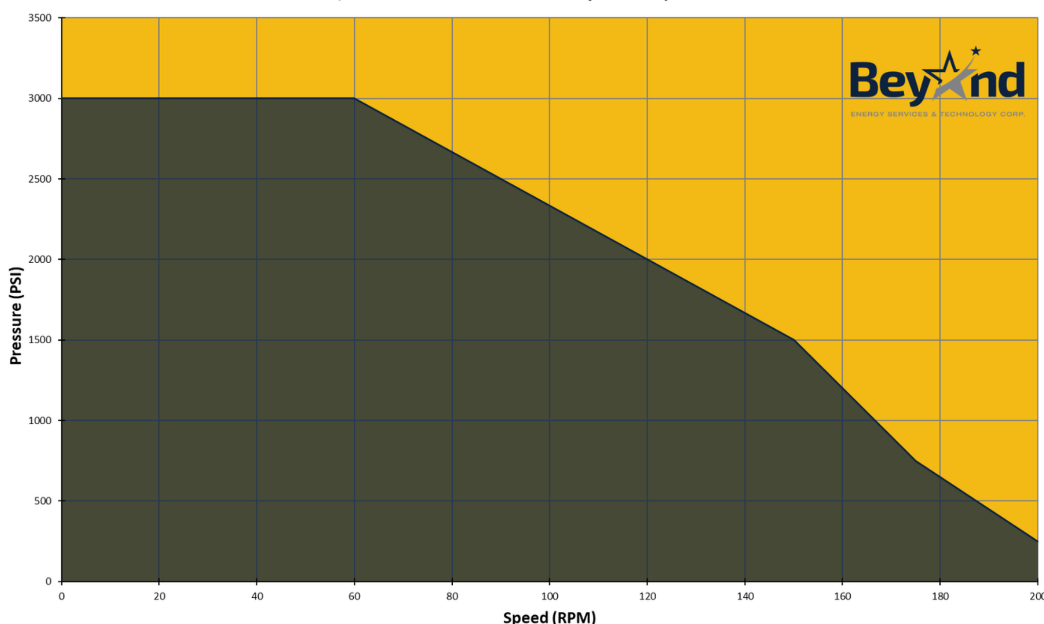
ARES 3090/POSEIDON 3090 Maximum Dynamic Operational Limits
